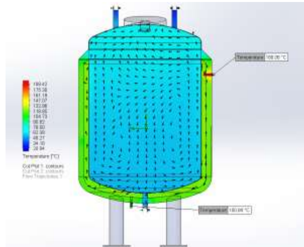
Figure 10. Fluid inlet and outlet temperature (jacket)
