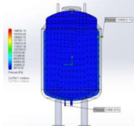
Figure 7. Steam inlet and outlet pressure (jacket)
