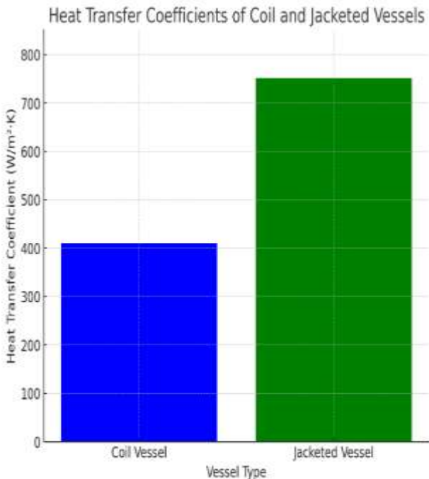
Figure 13. Heat transfer coefficient of coil and jacketed vessels
