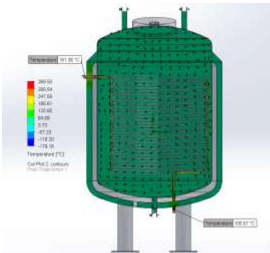
Figure 8. Steam inlet and outlet temperature (coil)
