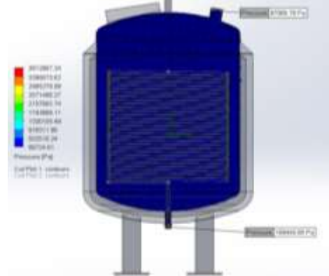
Figure 5. Fluid inlet and outlet pressure (coil)
