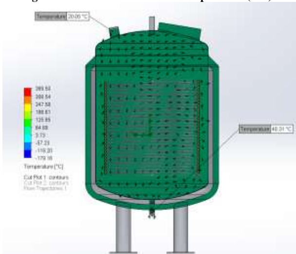
Figure 9. Fluid inlet and outlet temperature (coil)
