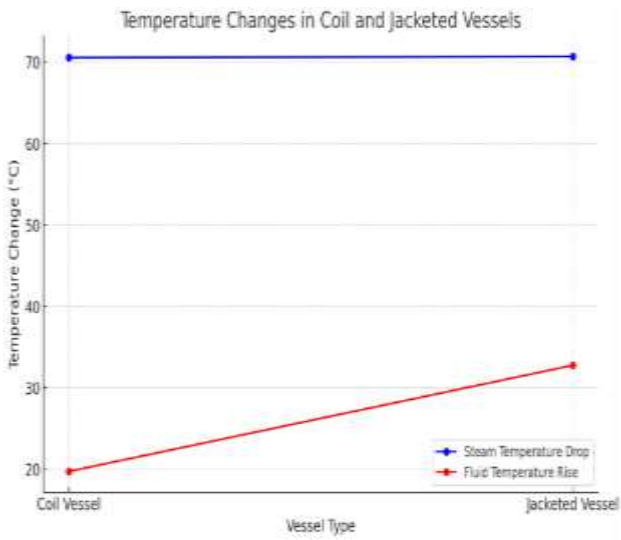
Figure 12. Temperature changes in coil and jacketed vessels
